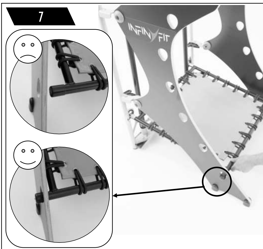
Push on the trampoline to check it's properly secure.
